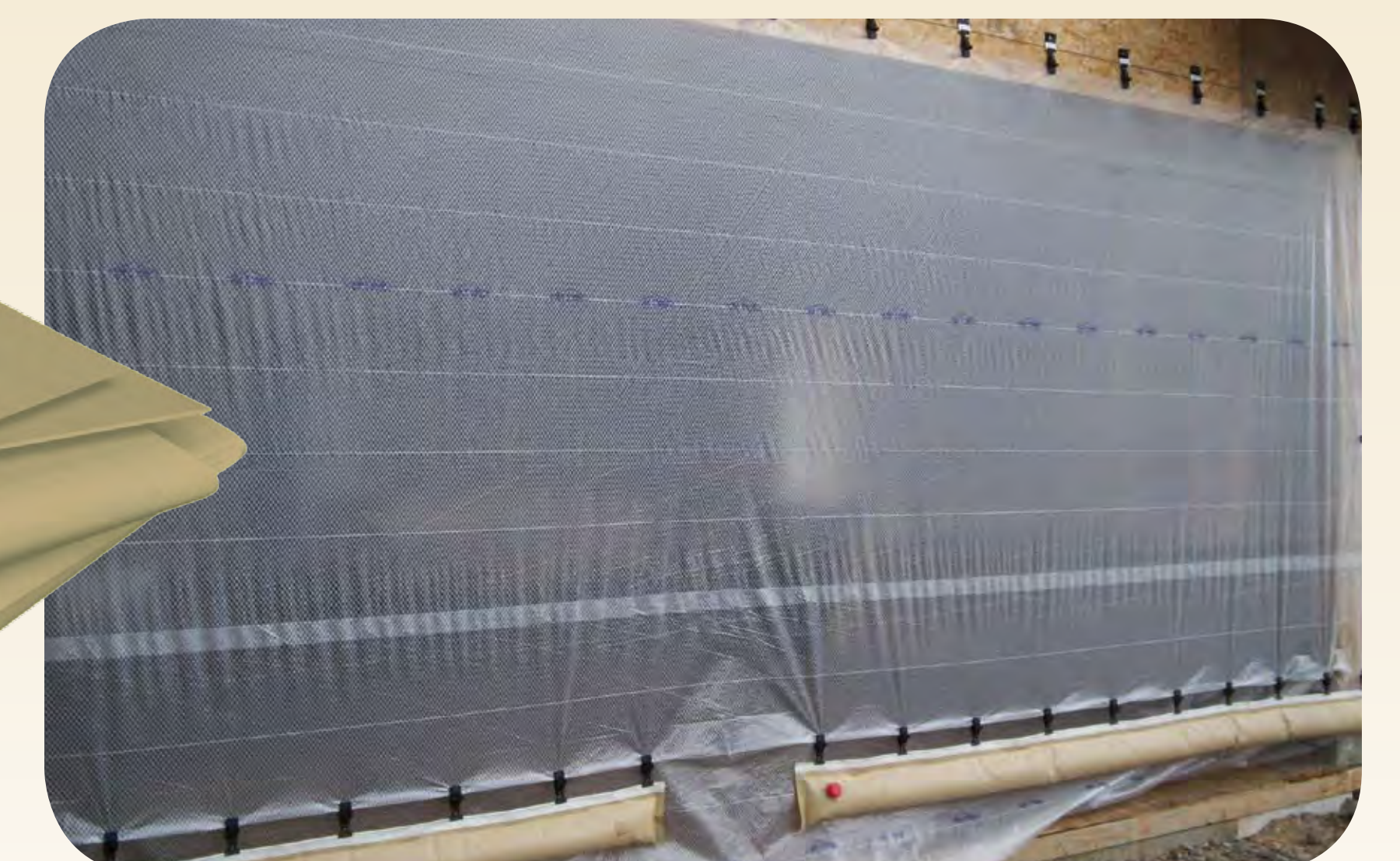
Close-in open spaces for Weather Protection Top is held with roll clips at 1 foot intervals
